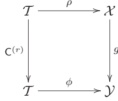
Figure 4.1: A commutative diagram representing a distinguishing property on C^r
