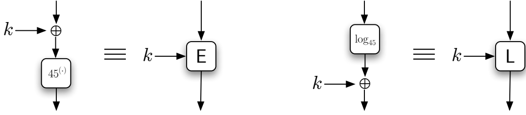
Figure 9.2: Replacing key exclusive-or and fixed substitution boxes by equivalent keyed substitution boxes
