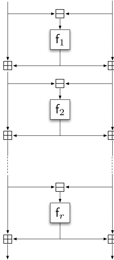
Figure 3.2: An r -round Lai-Massey scheme
